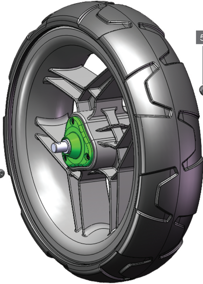
* 6 FRONT WHEEL ASSEM P1S-61##-FWASSM
